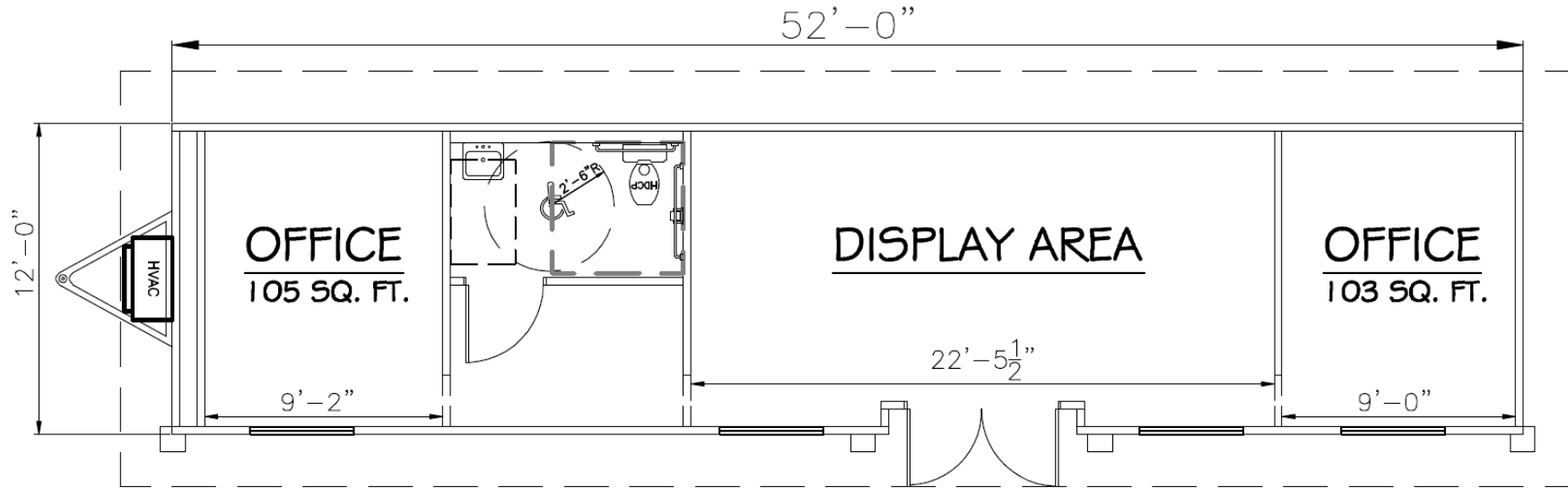
FLOOR PLAN
